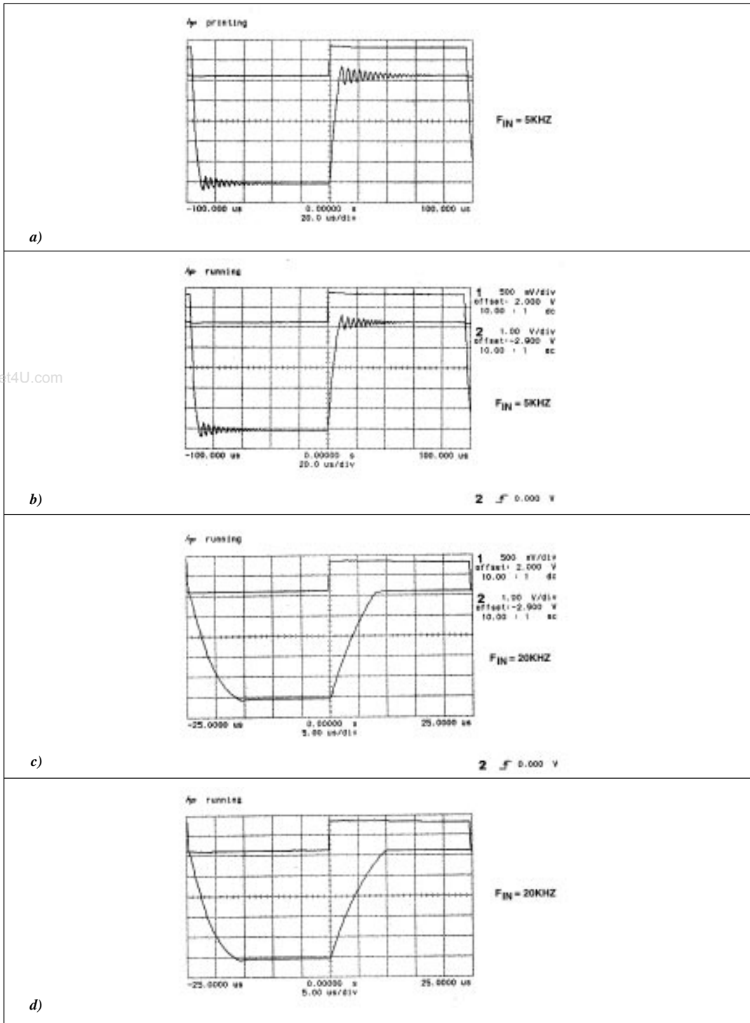
Plot 23. Pulse Response — a) C_{LOAD} = 47,000pF ; b) C_{LOAD} = 47,000pF , R_{LOAD} = 1kOhm ; c) 15 Ohms in series with C_{LOAD} = 47,000pF ; d) R_{LOAD} = 1kOhm , 15 Ohms in series with C_{LOAD} = 47,000pF .
