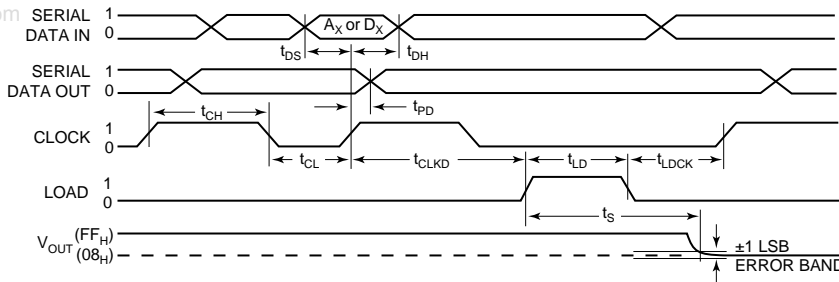
SERIAL DATA INPUT TIMING DETAIL (PRESET = Logic "1"; V_{IN(X)} = 1.5V ; V_{REFL} = 0V )
